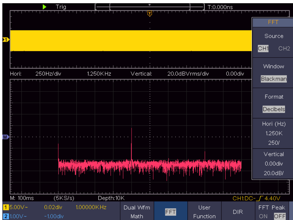
Figure 4-3 Blackman window
