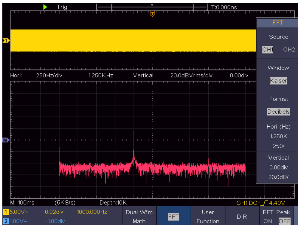
Figure 4-5 Kaiser window
