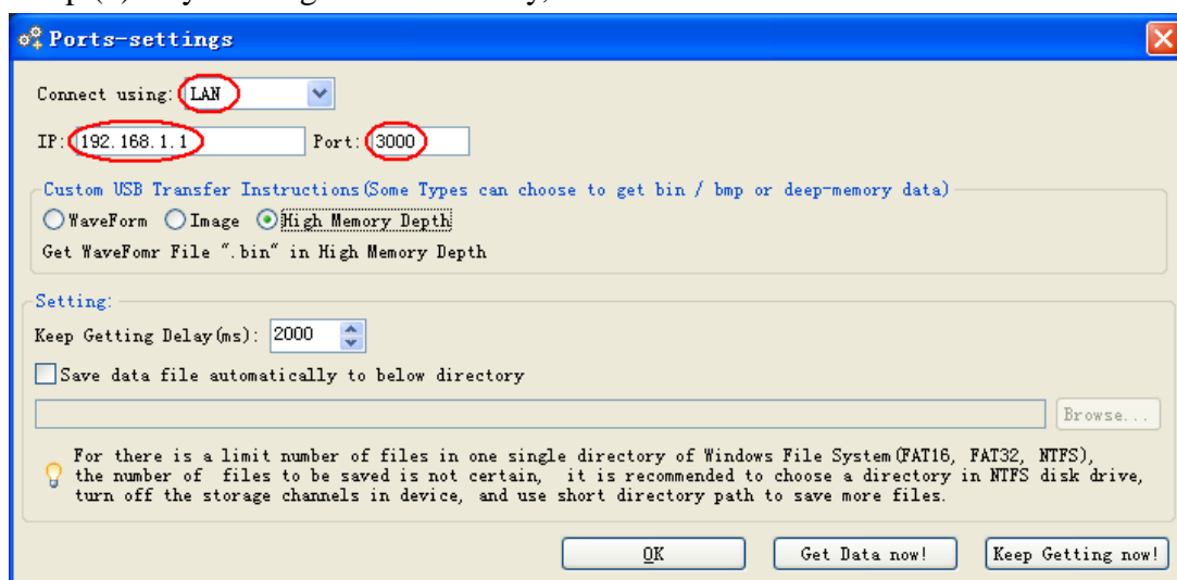
Figure 6-7 Set the network parameters of the Oscilloscope Software
