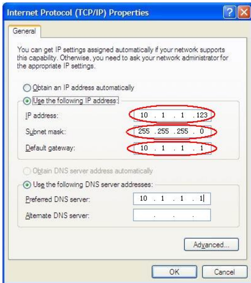
Figure 6-8 Set the network parameters of the computer
