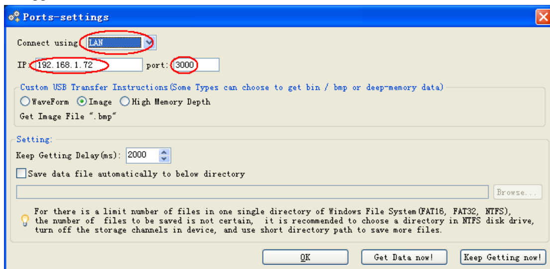
Figure 6-5 Set the network parameters of the Oscilloscope Software
