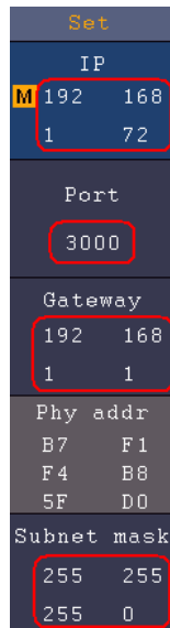
Figure 6-6 Set the network parameters of the oscilloscope
