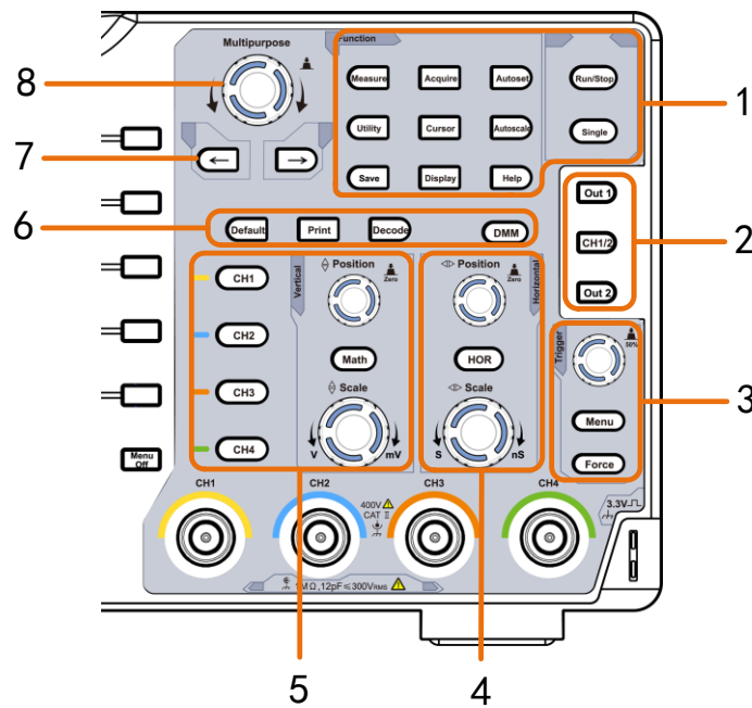
Figure 3-3 Control Area Overview
