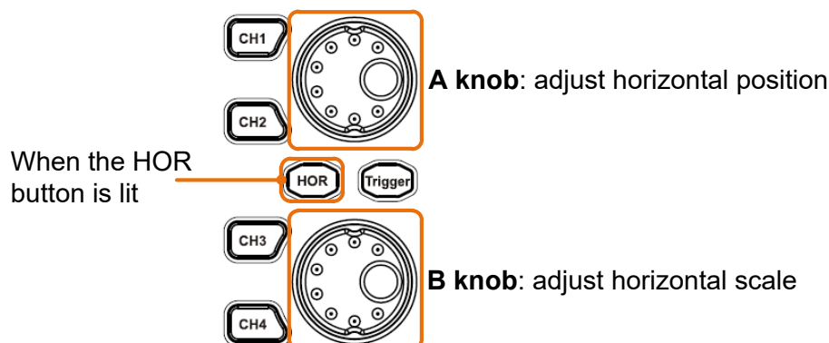
Figure 3-11 Horizontal Control
