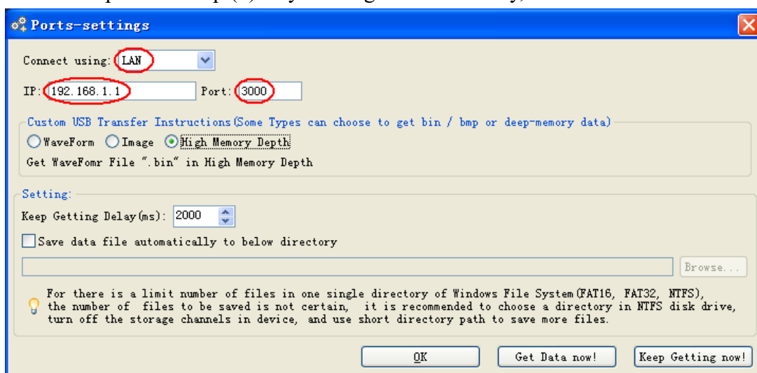
Figure 4-8 Set the network parameters of the OWON Oscilloscope Software
