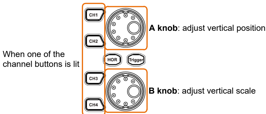
Figure 3-10 Vertical Control
