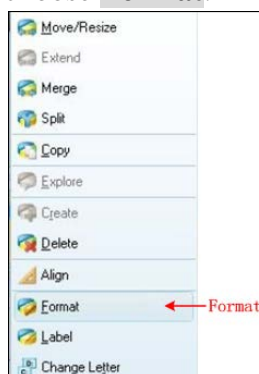
Figure 5-43: Choose format
