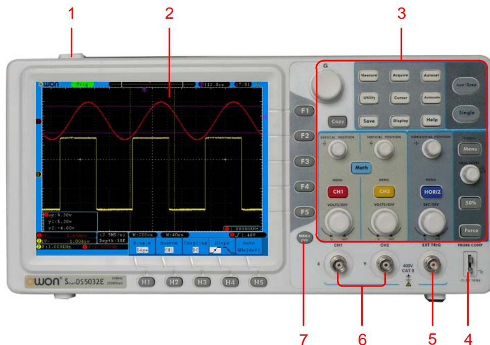
Figure 3-1 Front panel
